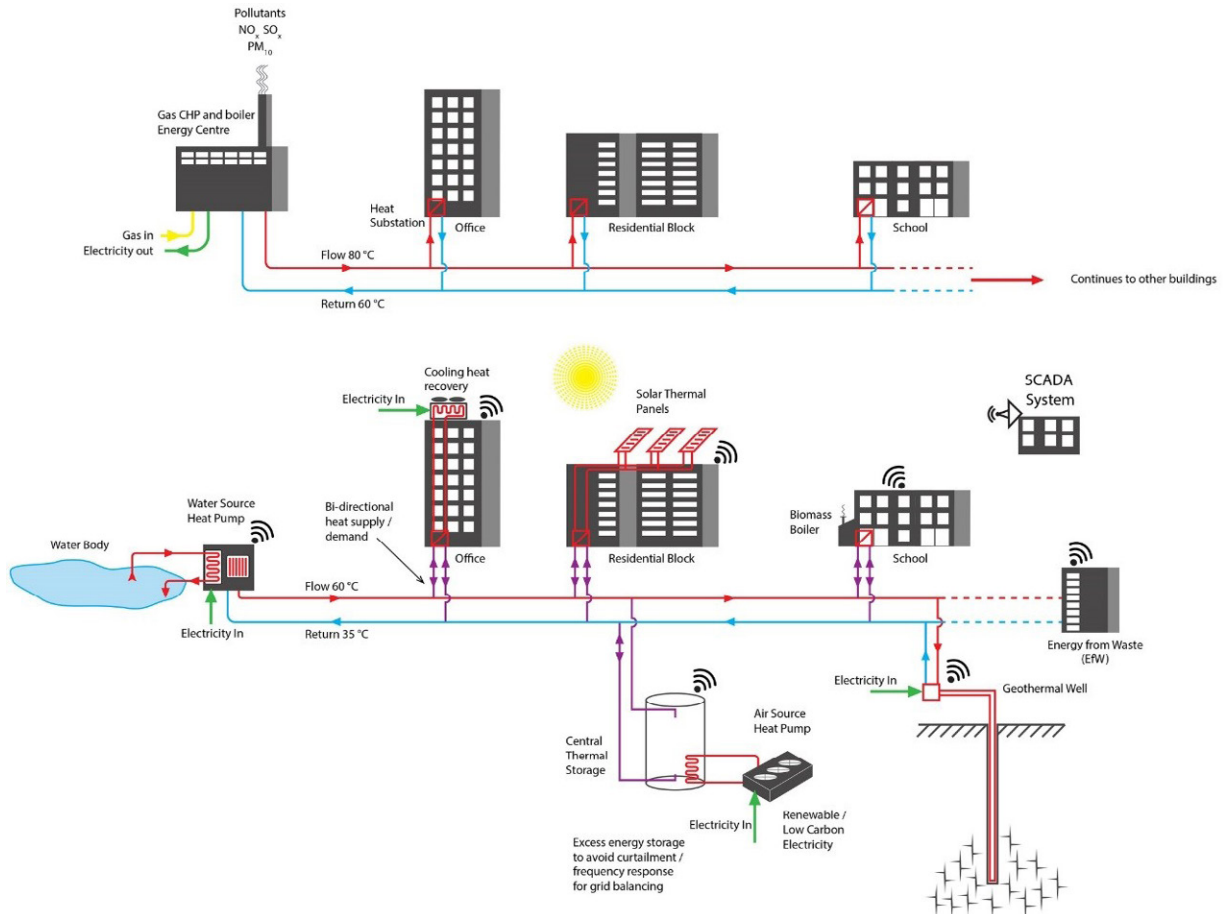
Figure 3 Integrated heat networks using multiple heat sources
